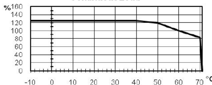
Output derating Curve Continuous Load
