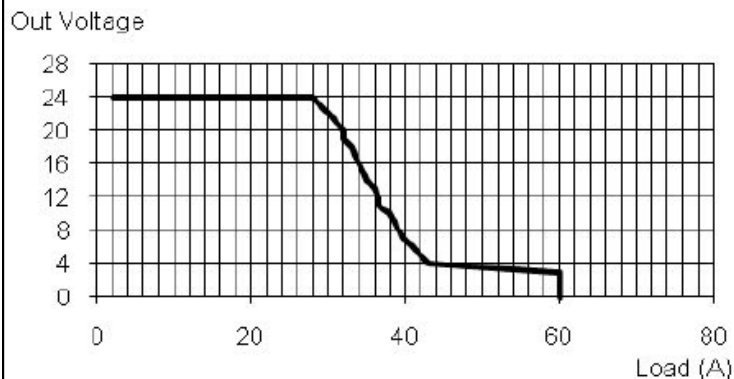
Output Voltage vs. Output Current, typ.
